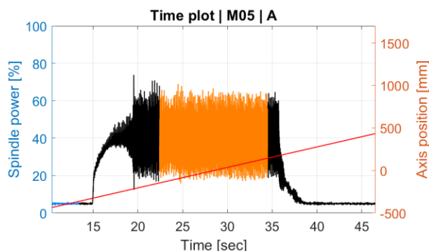
Figure 5: Example of the specific machining operation monitoring – a time-domain plot of spindle power and X axis position.
