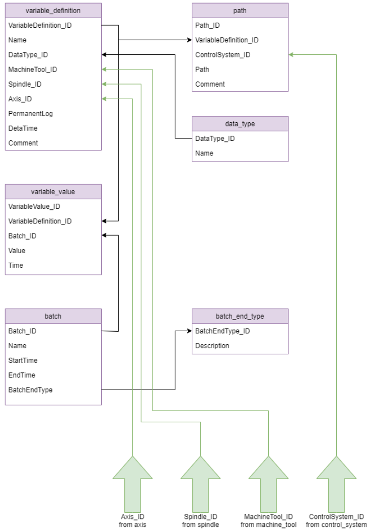
Figure 1d: Schema of the framework for milling process monitoring: the data model for the operation monitoring.
