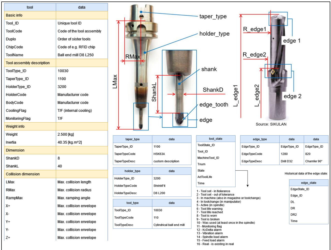
Figure 2: Example of the cutting tool components and their description within the proposed framework.
