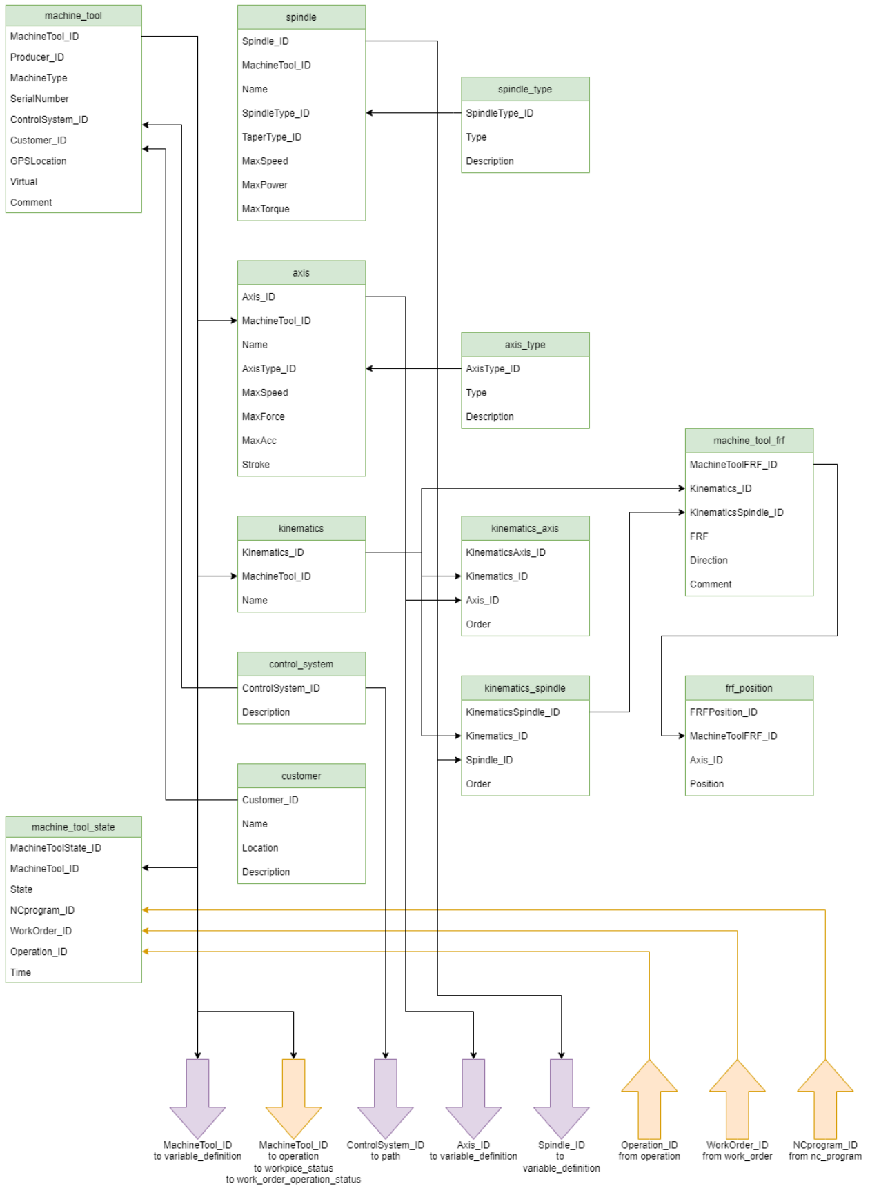
Figure 1b: Schema of the framework for milling process monitoring: the data model for the machine tool.
