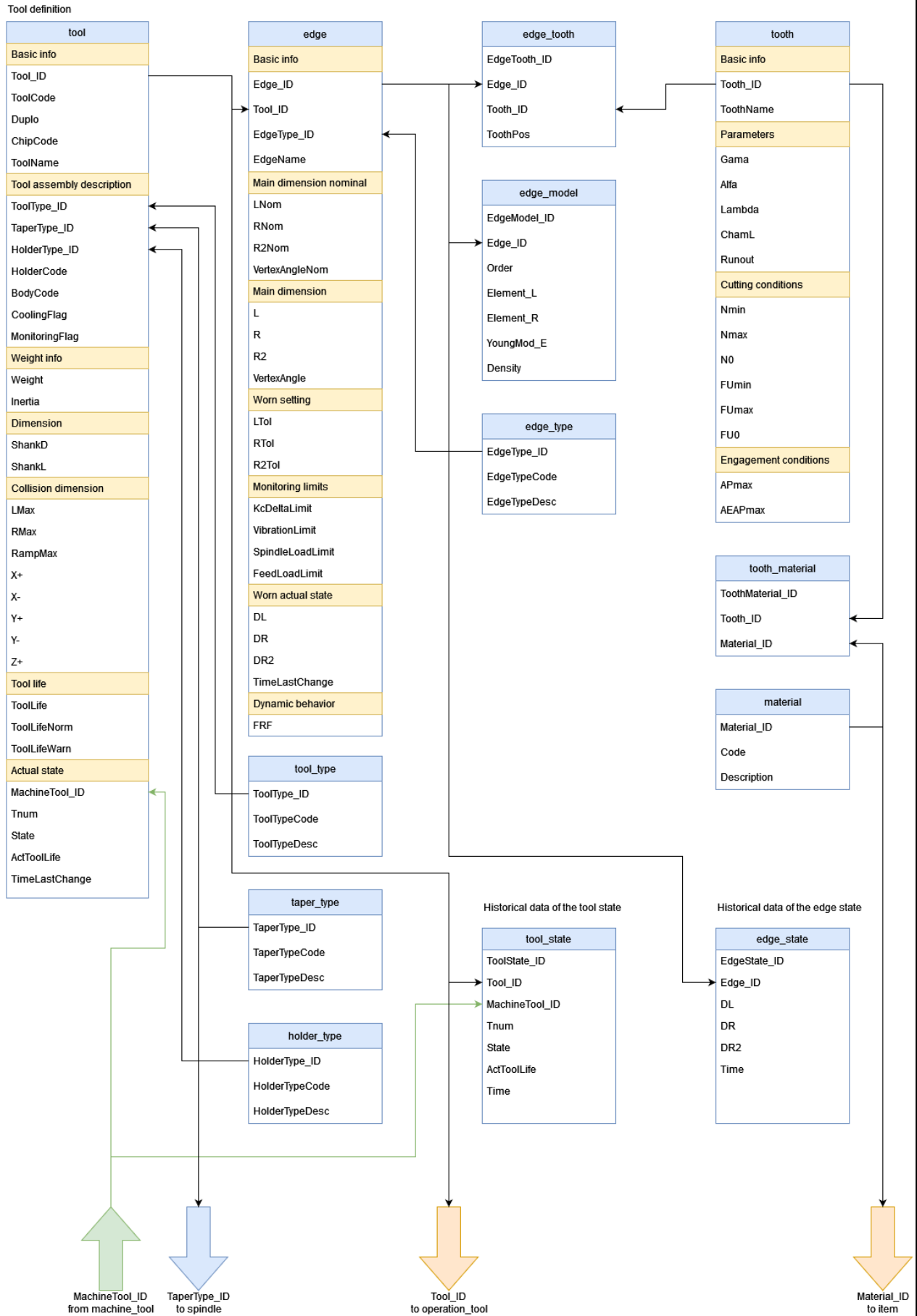
Figure 1a: Schema of the framework for milling process monitoring: the data model for the tool.
